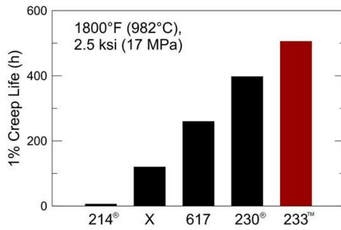
Comparative Time to Produce 1% Creep (Sheet)
